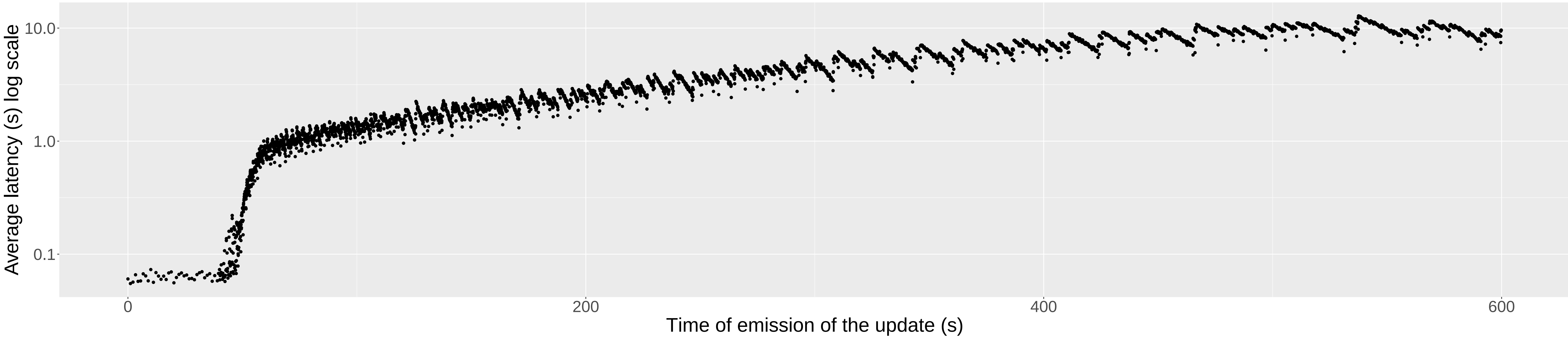
Classical Op-based 20/20 Peers/Peers Updating, 1k Updates
